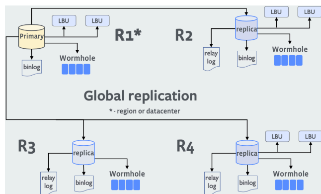
Figure 2: UDB Architecture
