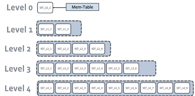
Figure 3: RocksDB Architecture
